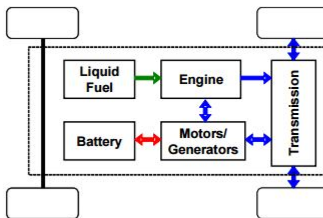
Schematic of a series-parallel hybrid powertrain Source:
